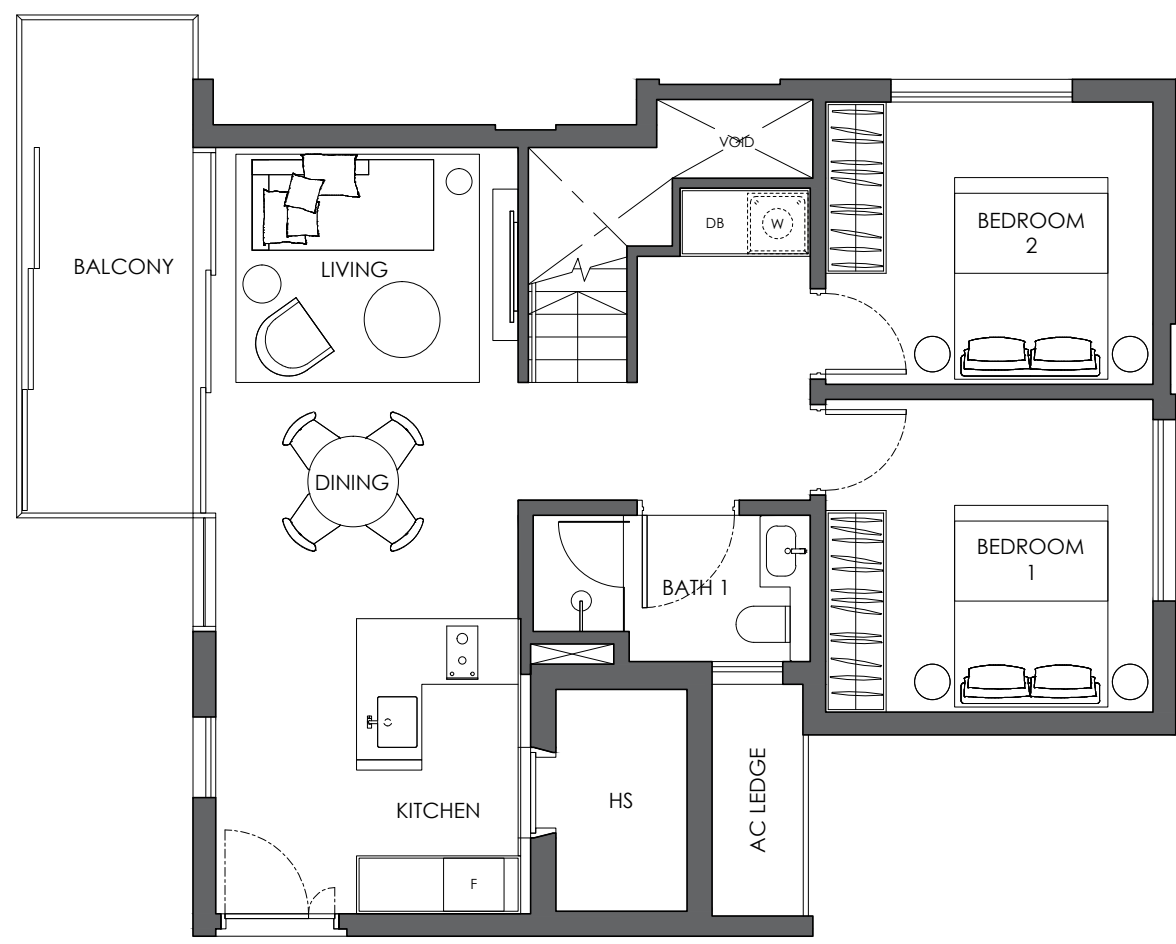
5TH STOREY PLAN
