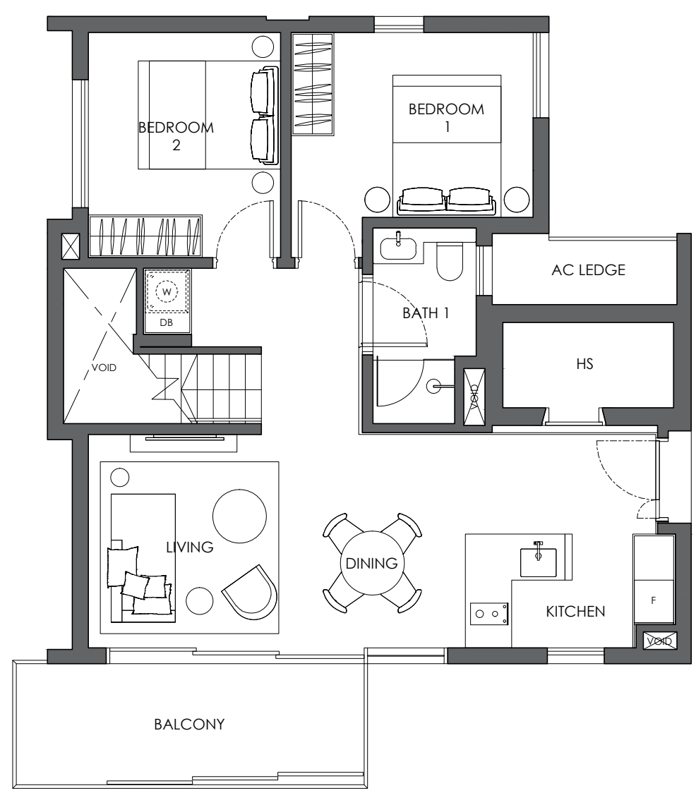
5TH STOREY PLAN
